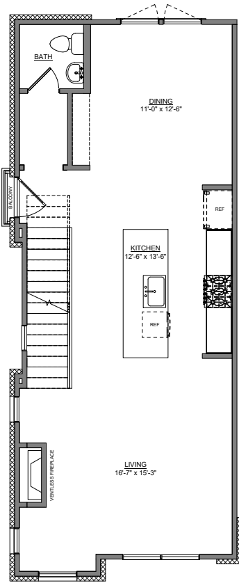
FLR - LEVEL 02 - UNIT 13 ATHENS - END UNIT
