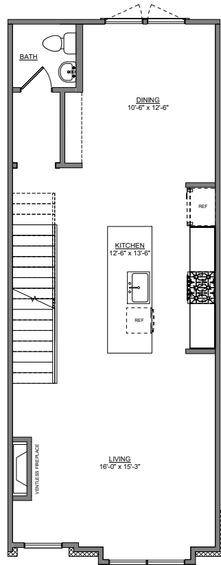
FLR - LEVEL 02 - UNIT 11 MILAN - MIDDLE UNIT
