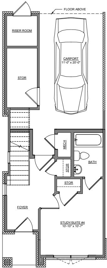
FLR - LEVEL 01 - UNIT 13 ATHENS - END UNIT
