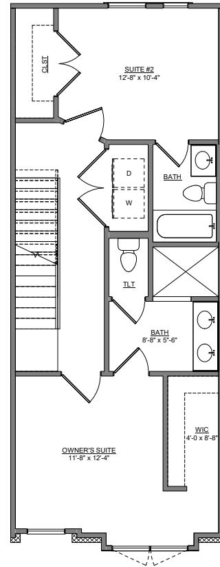
FLR - LEVEL 03 - UNIT 11 MILAN - MIDDLE UNIT
