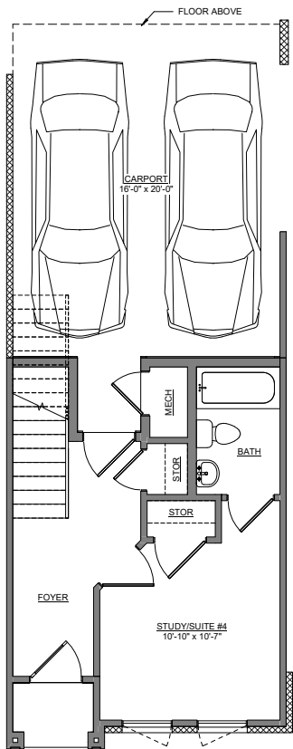
FLR - LEVEL 01 - UNIT 10 BRISTOL - MIDDLE UNIT
