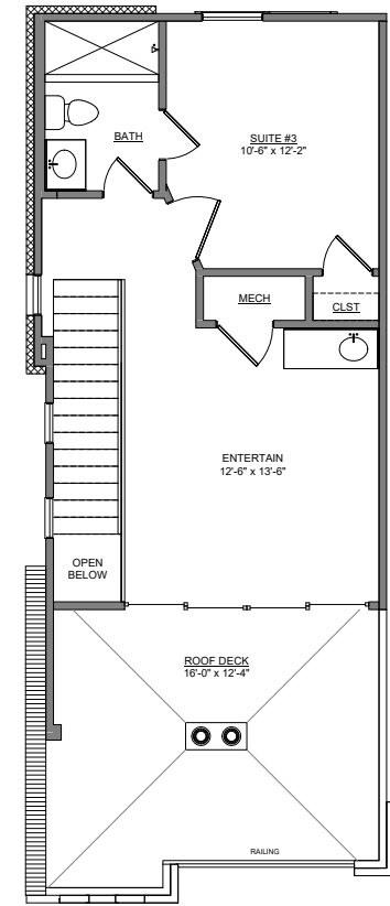
FLR - LEVEL 04 - UNIT 13 ATHENS - END UNIT
