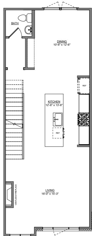
FLR - LEVEL 02 - UNIT 12 PARIS - MIDDLE UNIT
