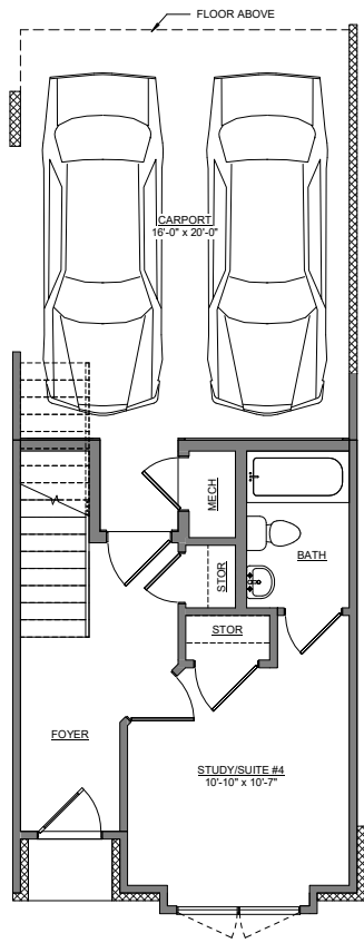
FLR - LEVEL 01 - UNIT 11 MILAN - MIDDLE UNIT
